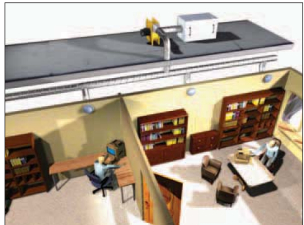
Displacement Ventilation
